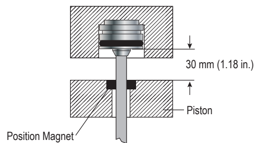
Magnet installation in non-ferrous material
