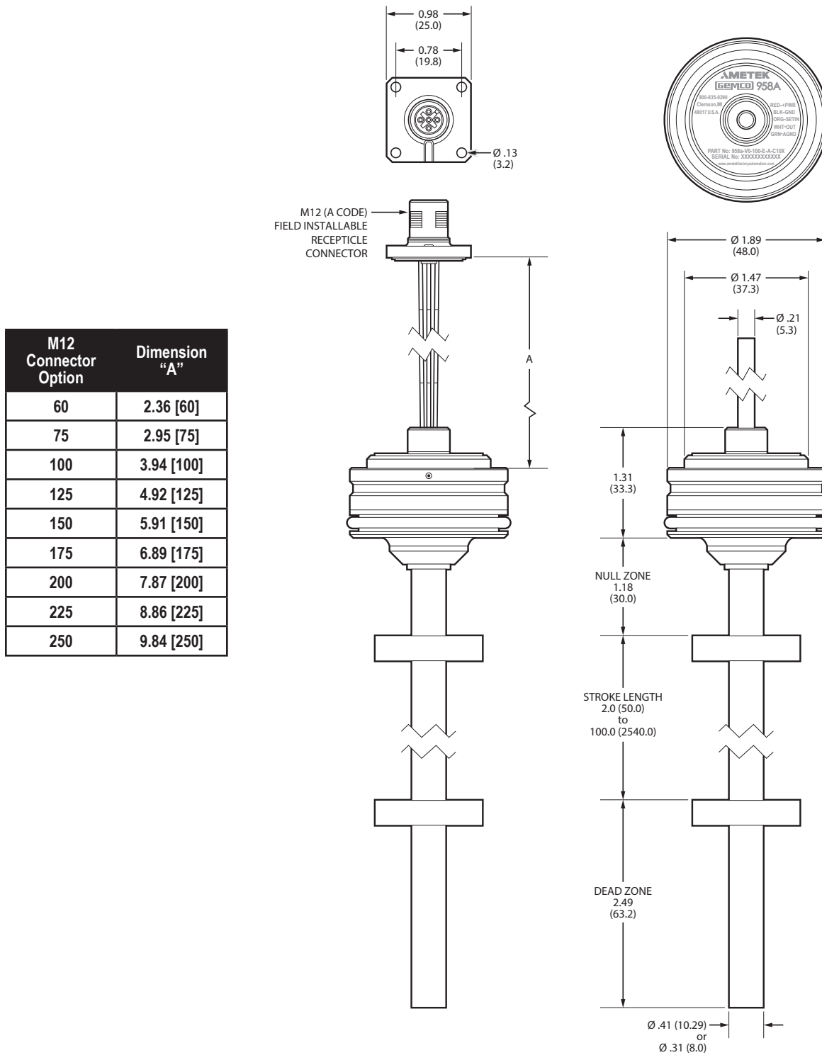
Figure 1-1: 958A Dimension Drawing (PD-0126000)
